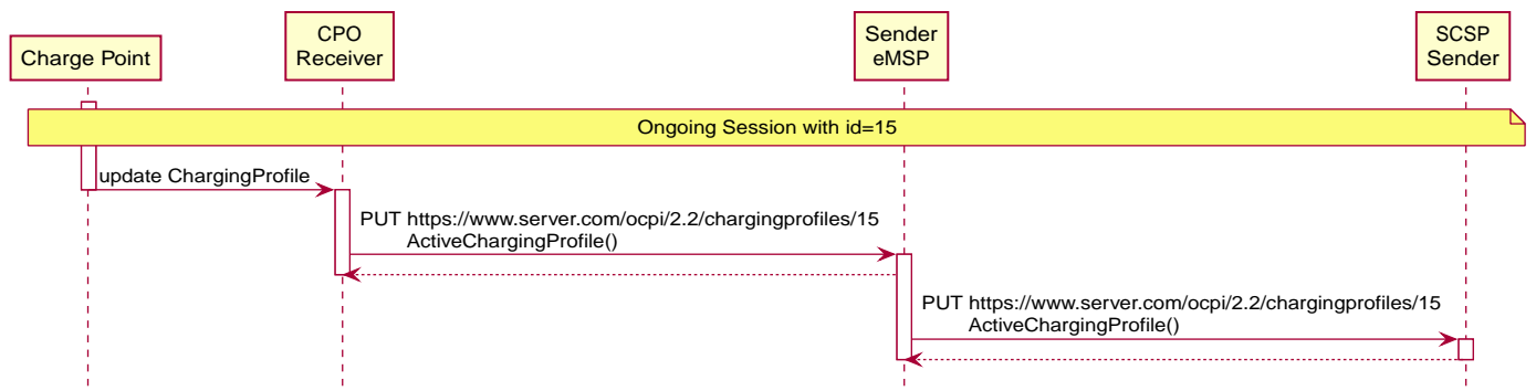
Figure 46. Example of an ActiveChargingProfile being sent by the CPO via the eMSP
