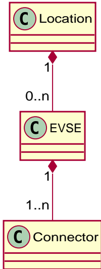
Figure 24. Location class diagram
