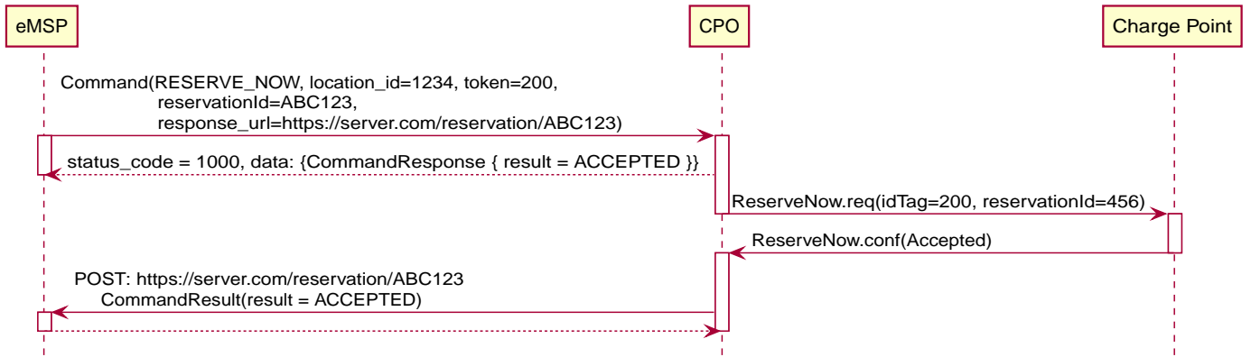
Figure 34. Successful RESERVE_NOW
