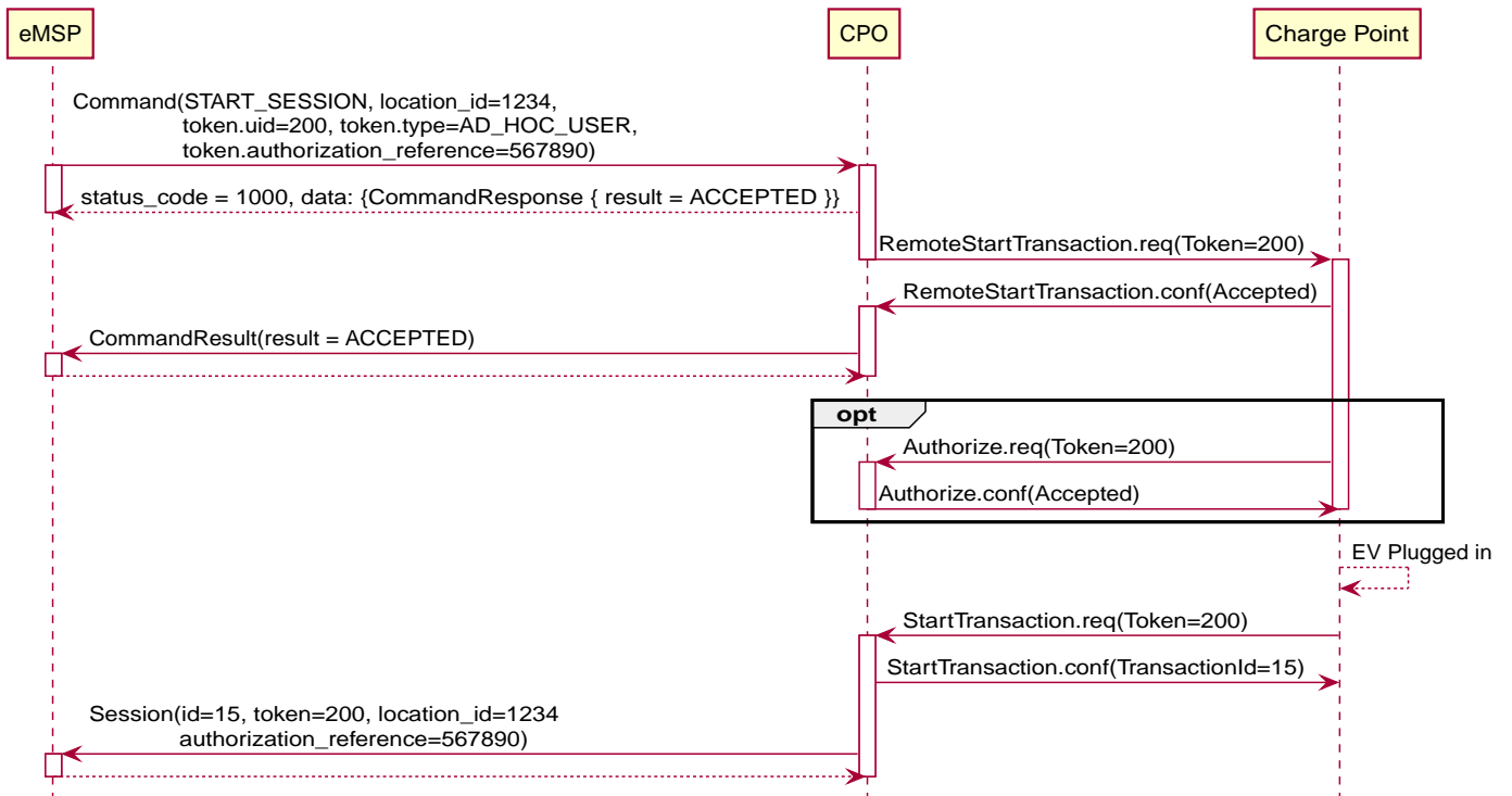
Figure 30. START_SESSION successful
