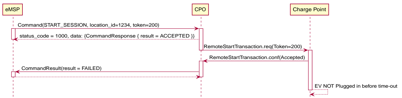
Figure 28. START_SESSION failed
