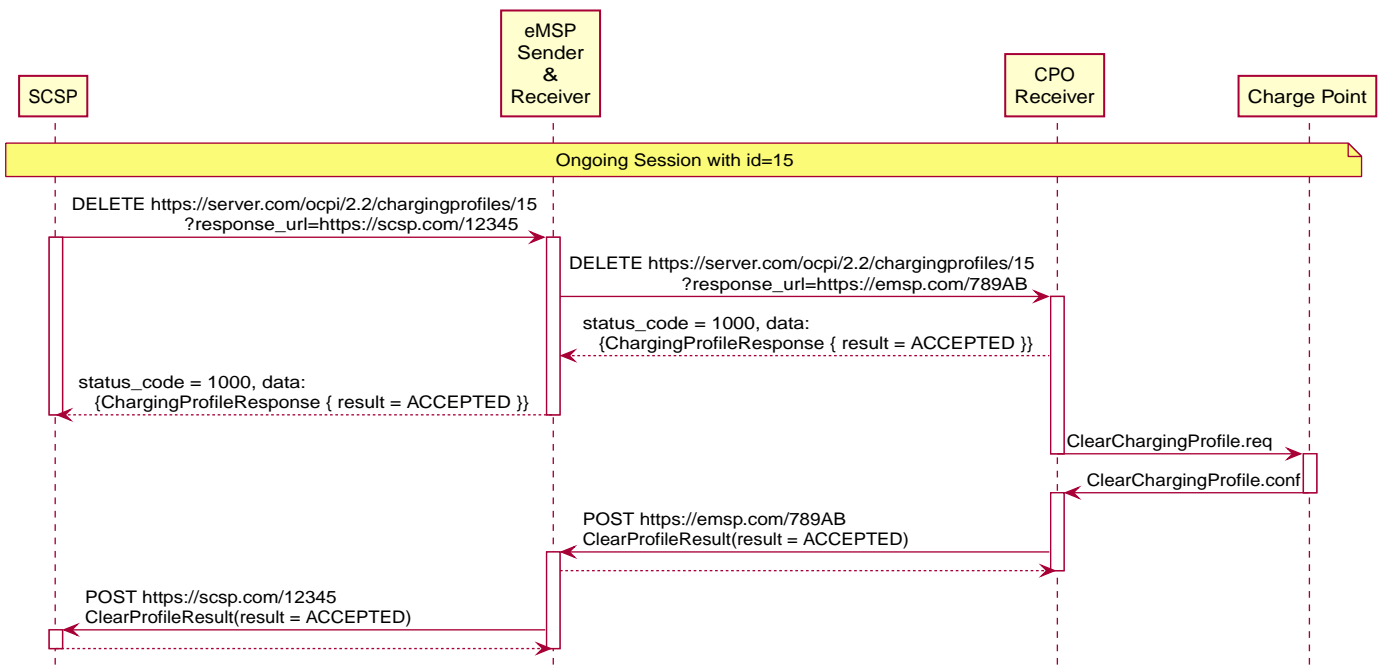
Figure 42. Example of a ClearChargingProfile via the MSP.
