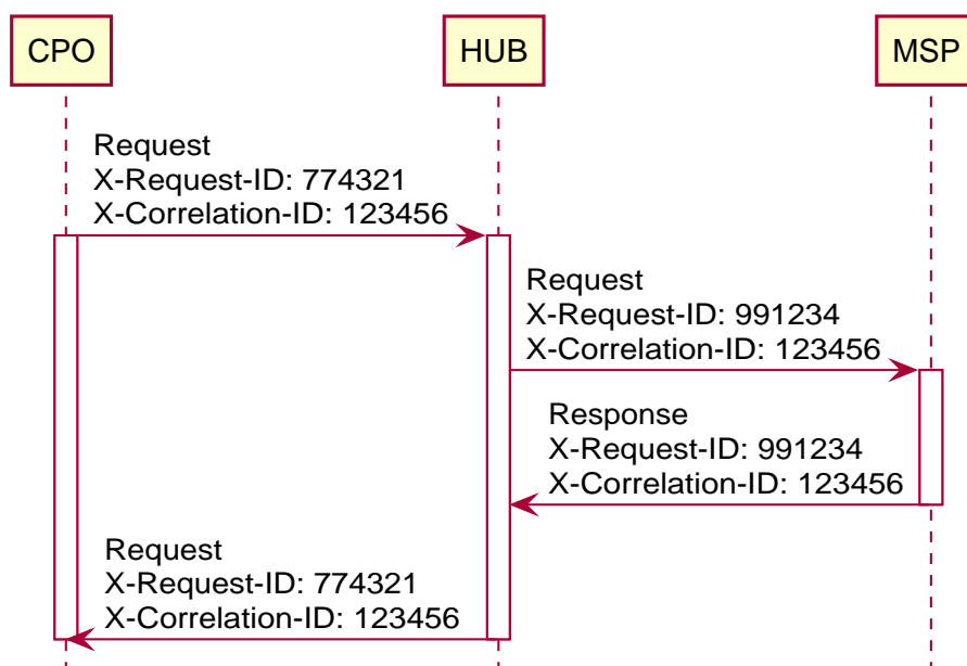
Figure 21. Example sequence diagram of the uses of X-Request-ID and X-Correlation-ID in a topology with a Hub.
