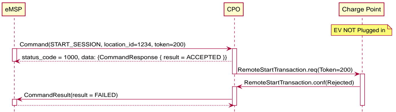
Figure 29. START_SESSION failed
