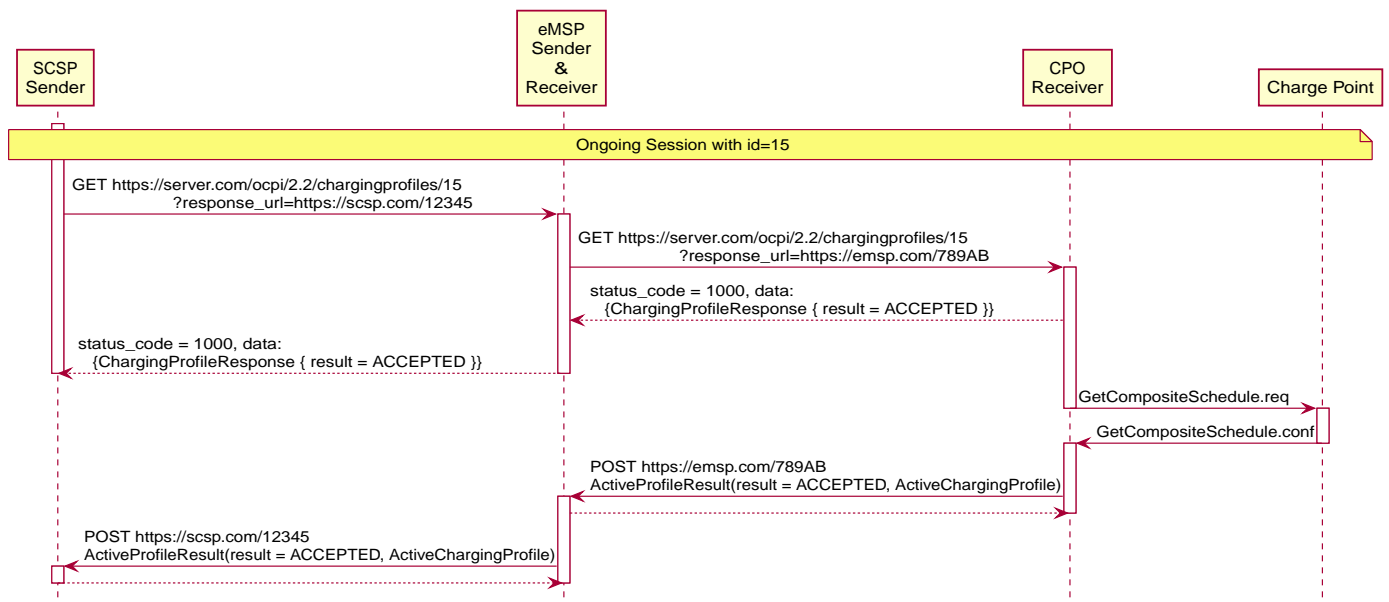
Figure 44. Example of a GET ActiveChargingProfile via the MSP.
